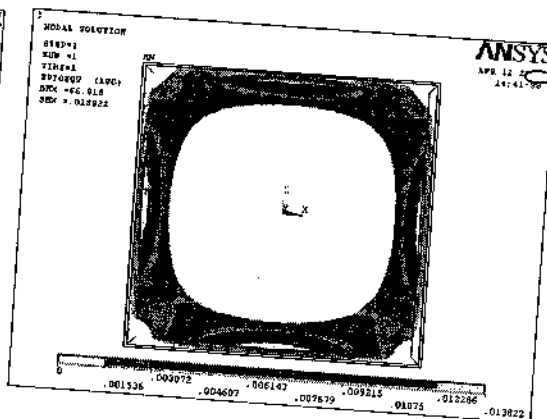
Fig: Strain plot for bottom flat SMC panel
