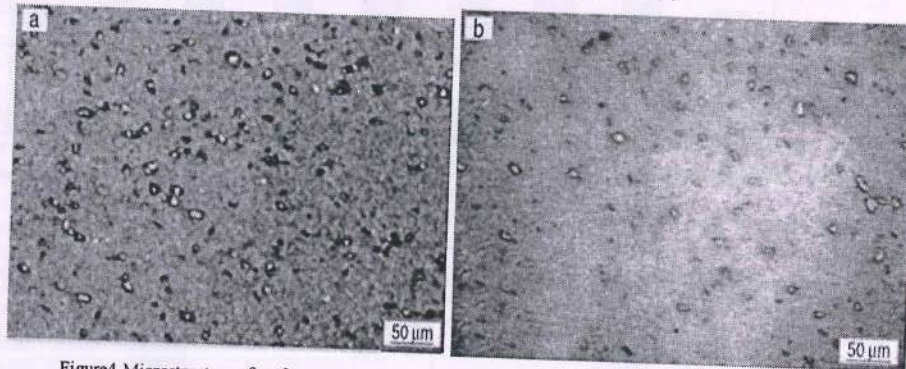
Figure 4. Microstructure of surface hybrid composites (a) Al-SiC/Gr; (b) Al-SiC/Al 2 O 3 (Deravaju et al. [5])
