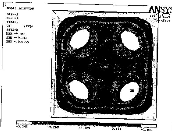
{Fig: Deflection plot for a bottom SMC concave panel fig: Deflection plot for a bottom SMC convex panel
