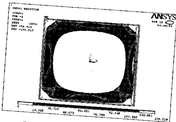
Fig: stress plot for a bottom flat SMC panel
