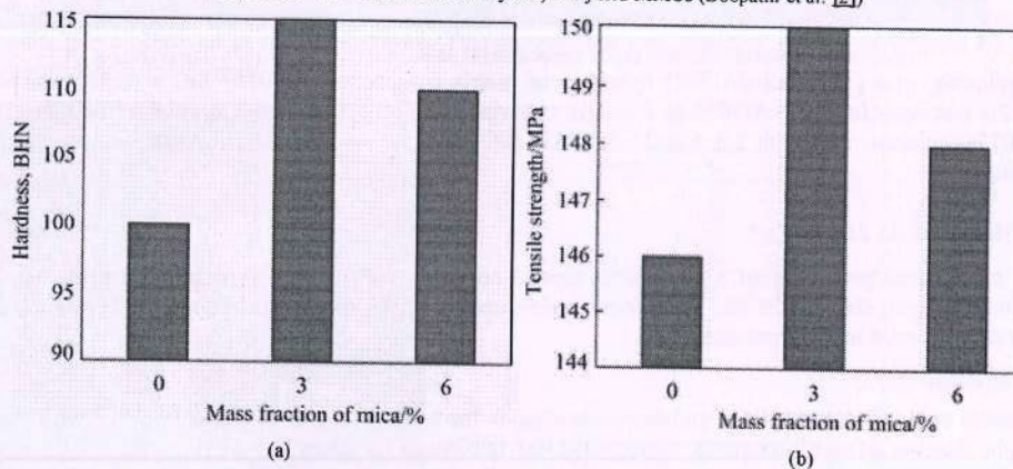
Figure 6. (a) Hardness (b) tensile strength of composite with different percentage of mica (Rajmohan et al. [3])
