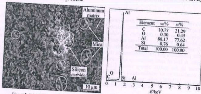
Figure 2. (a) SEM image of Al/10SiC-3mica composite (b) EDS spectrum of Al/10SiC-3mica composites (Rajmohan et al. [3])
