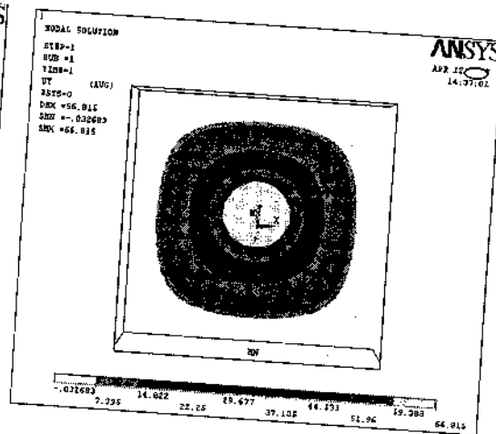
Fig: Deflection Plot for A Bottom Flat SMC Panel
