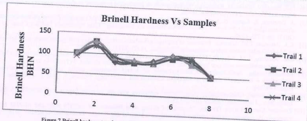
Figure 7. Brinell hardness test for Al 7075 hybrid metal matrix composites (Suryakumari et.al [11])
